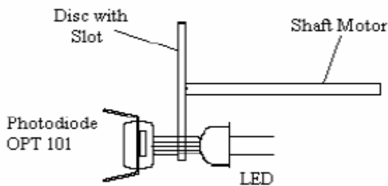
Fig 4 speed sensing
