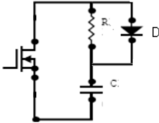
Fig 3 snubber circuit
