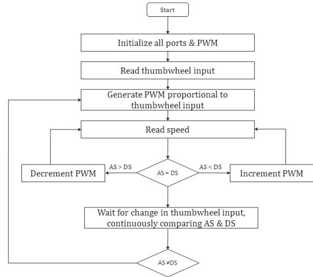
Fig 5 speed control program flow
