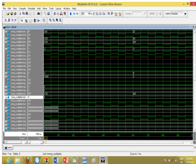
Fig.4. Simulation result of multiplier accumulate
