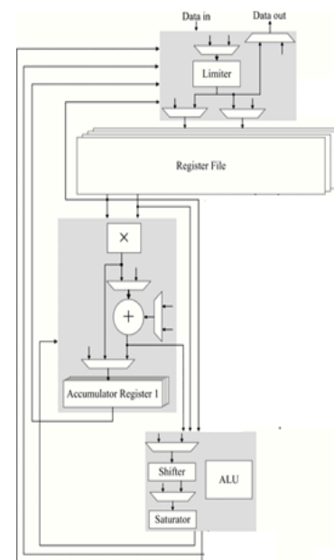
Fig.3. Proposed single MAC architecture
