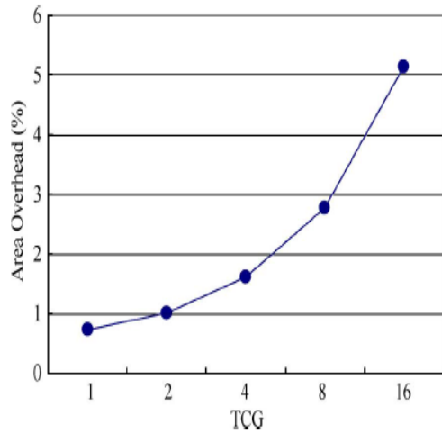
Fig. 7. Relation between TCG and area overhead
