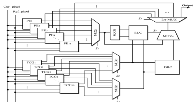
Fig. 6. Proposed EDDR architecture design for a ME. is
