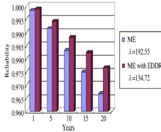
Fig. 9. Failure-rate and reliability analysis.
