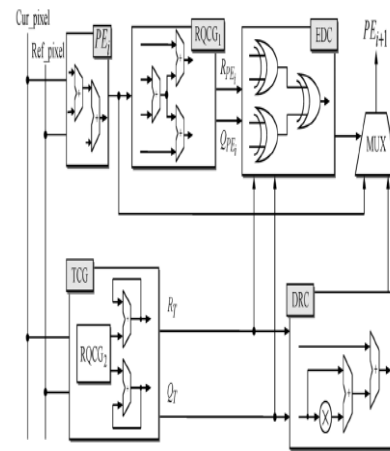
Fig. 2. A specific PE_i testing processes of the proposed EDDR architecture.
