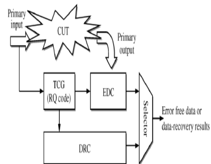
Fig. 1. Conceptual view of the proposed EDDR architecture.
