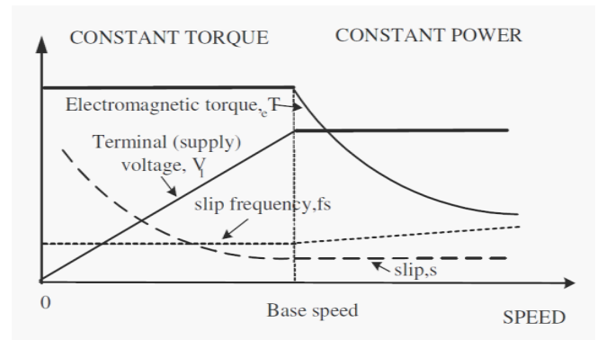
Fig. 6. Modes of operation of VVVF drives under V/ f control method.
