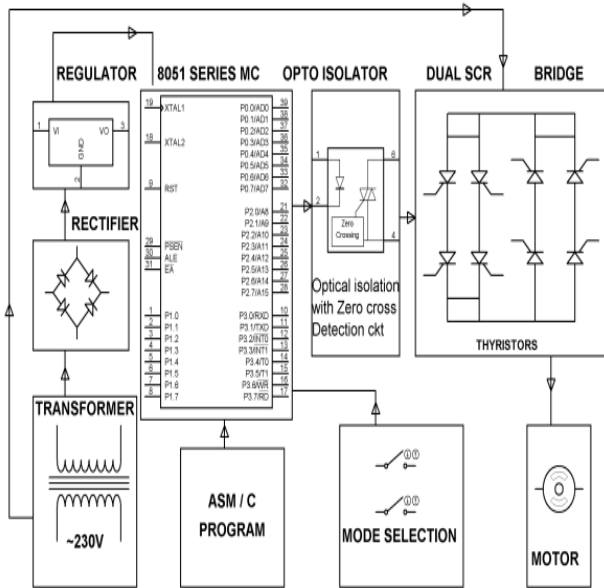
Fig.1 Schematic Diagram using Microcontroller
