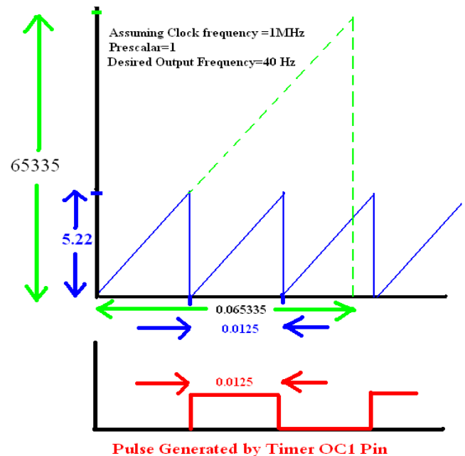
Fig.2. TIMER 1 pulse generation
