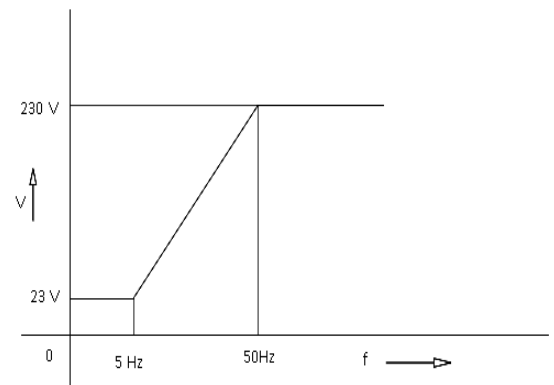
Fig. 6. Modes of operation of VVVF drives under V/ f control method.
