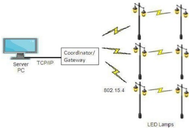
Figure 2.1. System Architecture
