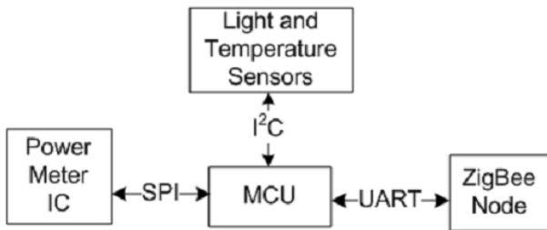
Figure 2.3. Block Diagram of the Controller
