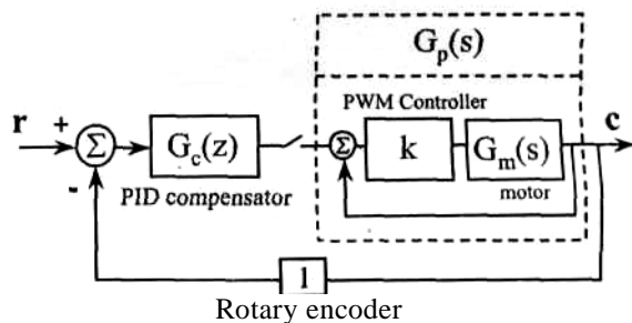
Figure 3 Schematic diagram of digital control
