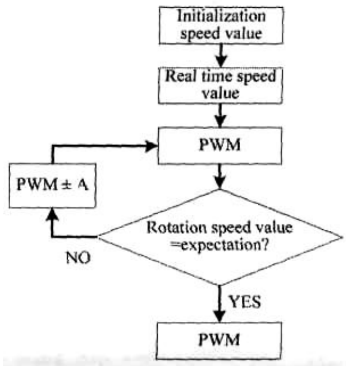
Fig. 4. Feedback control design
