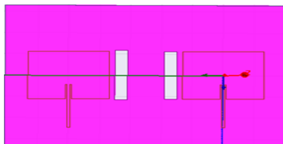
Figure 4: Microstrip Patch Array with two 0.06\lambda Rectangular Slots
