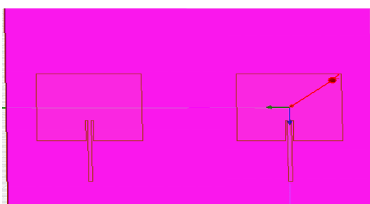
Fig 2: Microstrip Antenna Array without slots
