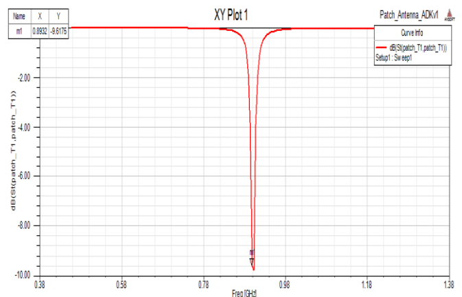
Fig 1: Return loss of an single antenna
