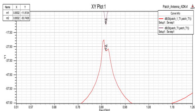
Fig 3: Return loss and S21 of Microstrip Antenna Array without slots
