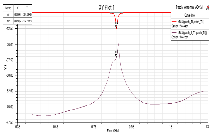
Fig 5: Return Loss and S21 of Microstrip Antenna Array with Slots
