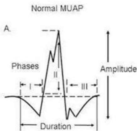
Fig 3 Characteristics Of Emg Signal
