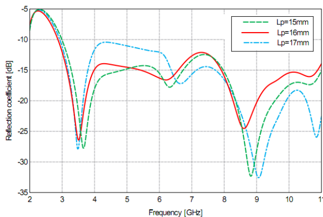
Fig.5 Return loss vs. frequency graph for different length of patch
