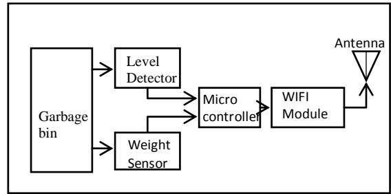
Fig. 1 Transmitter
