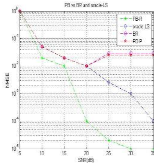
Fig. 1: Performance comparison of algorithms
