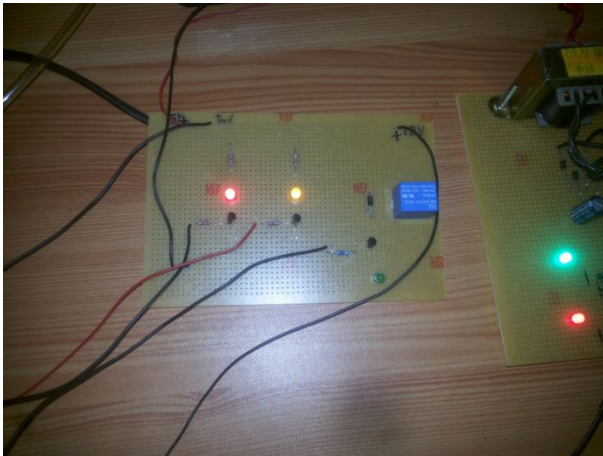
Figure 6: Yellow LED- Level 2 reached Indicating the tank is Half filled
