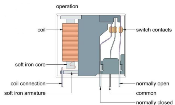
Figure 3: SPDT Internal Structure
