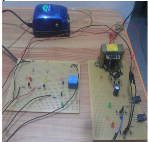
Figure 2: Hardware Kit Setup (PCBs with necessary components, Motor & Power Supply)
