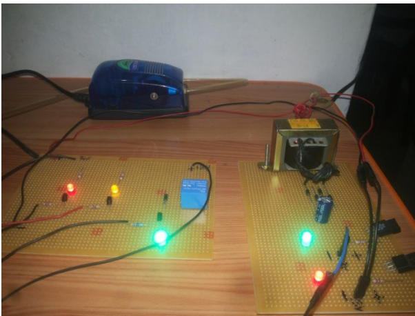
Figure 7: Green LED- Level 3 reached Indicating the tank is Completely filled
