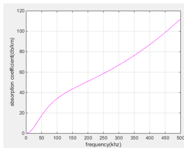
Fig 1. Absorption coefficient versus frequency : Implementation with Thorps' formula
