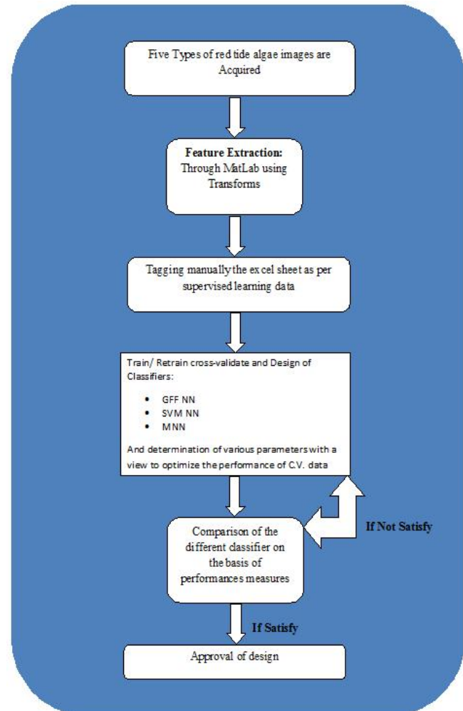
Figure.2 Methodology of work
